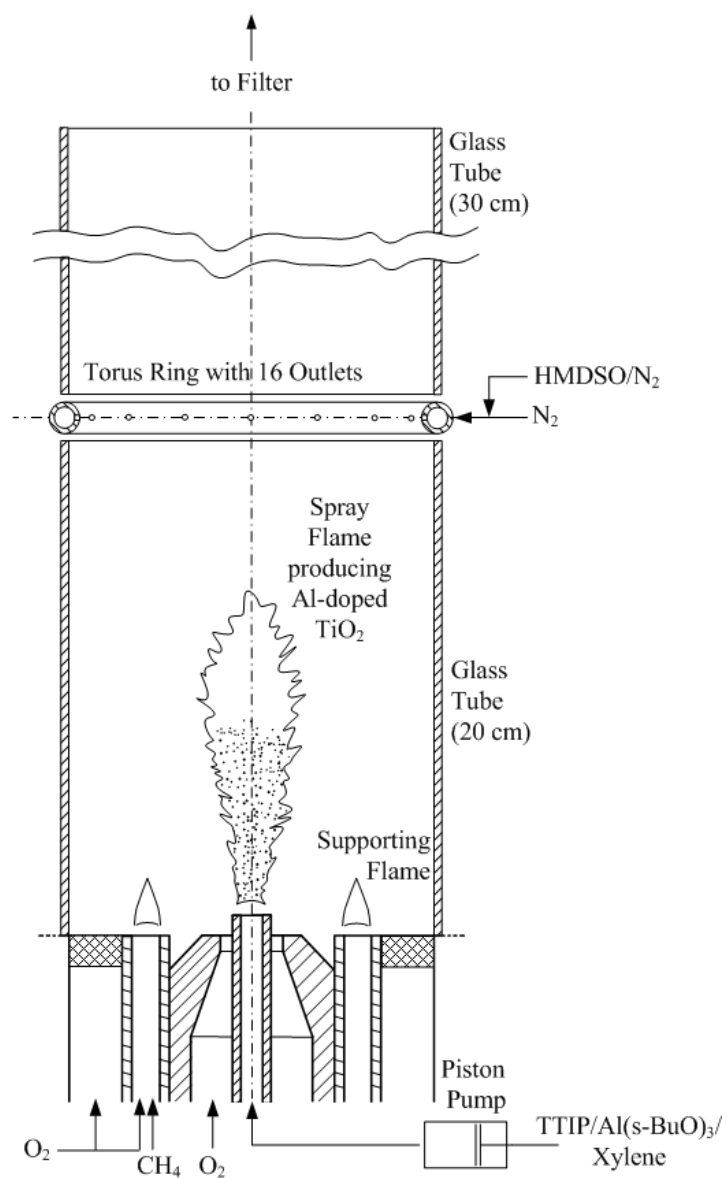
Figure S1. Experimental set-up for in-situ SiO 2 -coating of FSP-made Al/TiO 2 nanoparticles.
