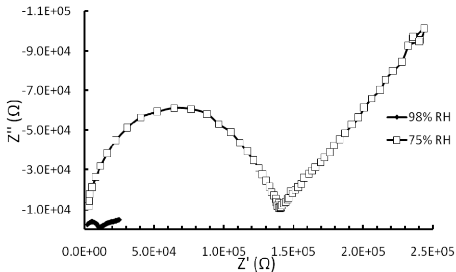
Figure S1. Representative Nyquist plots for the silica colloidal material. Shown are the plots for unmodified close-packed assembly at 75 and 98 % R.H.
