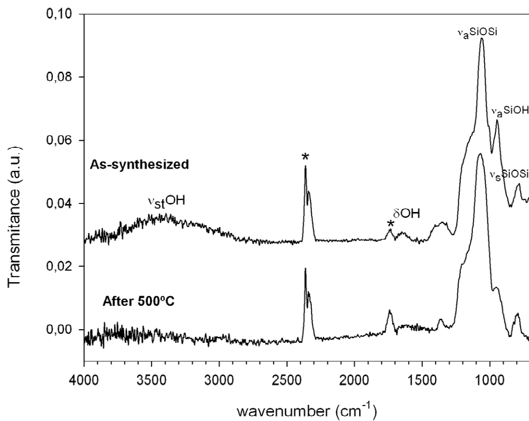
Figure A. ATR-FTIR spectra of as-synthesized and fired (500°C) EZS samples (asterisks: asymmetric and symmetric stretching modes of \text{CO}_2 from air).
