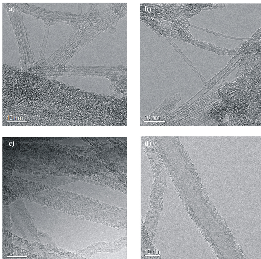
Figure S1. (a) Pristine SWNTs; (b) Nitric acid treated SWNTs; (c) Pristine MWNTs; (d) Nitric acid treated MWNTs.
