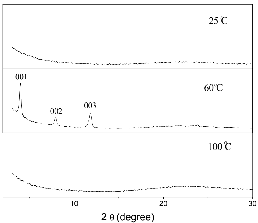
Fig. S2 X-Ray diffraction patterns of the thin film of 3 deposited on OTS/SiO 2 /Si substrate at various substrate temperatures ( T_{\text{sub}} )
