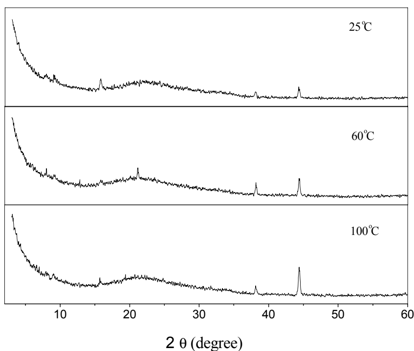
Fig. S1 X-Ray diffraction patterns of the thin film of 2 deposited on OTS/SiO 2 /Si substrate at various substrate temperatures ( T_{\text{sub}} )
