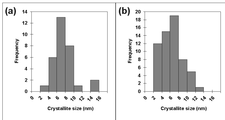
Figure 1. Particle size distribution for the primary nanoparticles in a) GDCNT1 and b) GDCNT2. Frequency refers to the number of measurements. Each particle was measured in two orthogonal directions.
