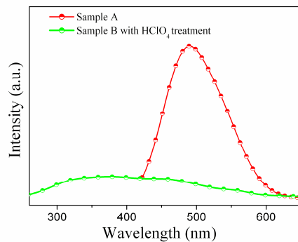
Fig. S1 PL spectra of sample B with \text{HClO}_4 treatment and sample A
