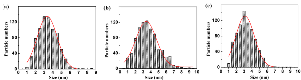
Fig. S2 Size distribution of CNPs in different samples, (a) in sample C, (b) in diamine hydrate, (c) in diethanolamine
