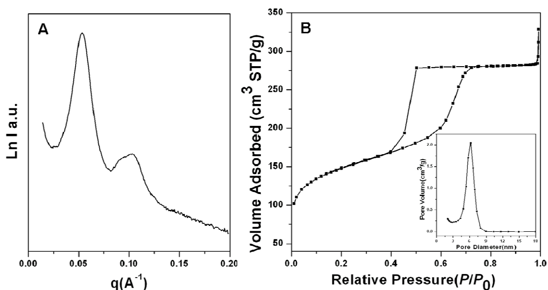
Figure S1. SAXS pattern (A), nitrogen adsorption-desorption isotherms (B) and corresponding pore size distribution (B, inset) of mesoporous siliceous \text{MSiO}_2 .
