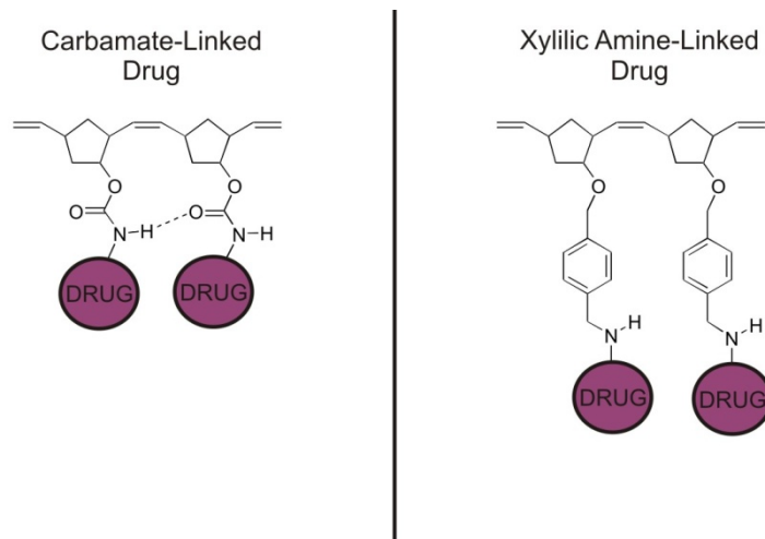
Fig. S1. (Left) Hydrogen bonding of the amine hydrogen to the carbonyl of the adjacent polymer unit. (Right) Xylylic amine hydrogens have no hydrogen bond acceptors.
