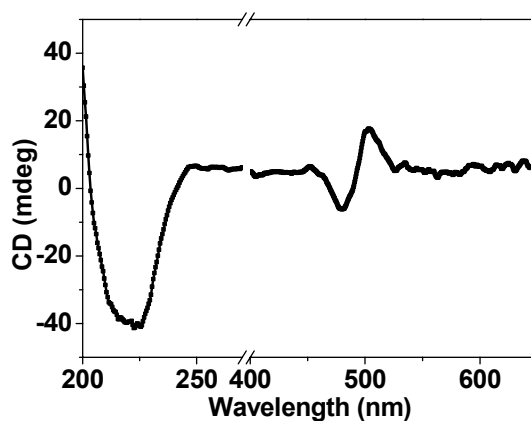
Figure S2 CD spectra of PLGA/PAH/SeCy (1mM) complex film after the treatment of HCl gas and vapor.
