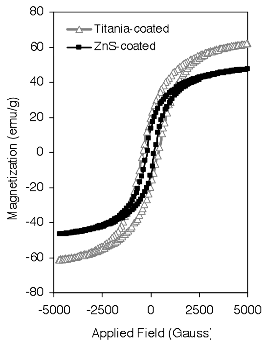
Figure S2. VSM hysteresis loops for titania- and zinc sulfide-coated hematite particles (measured at room temperature).
