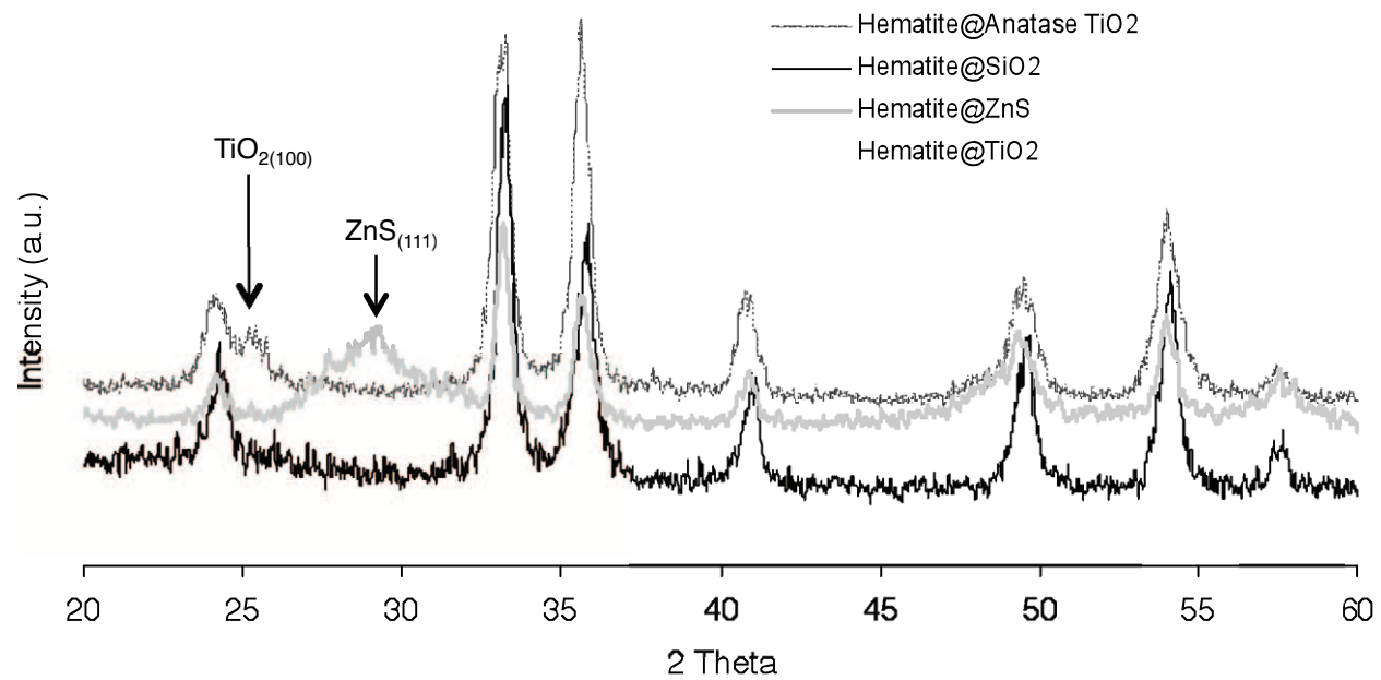
Figure S1. XRD pattern for various hematite core-shell samples (from top to bottom): \alpha -Fe 2 O 3 -TiO 2 (anatase), \alpha -Fe 2 O 3 -ZnS, \alpha -Fe 2 O 3 -SiO 2 , and \alpha -Fe 2 O 3 -TiO 2 (amorphous).
