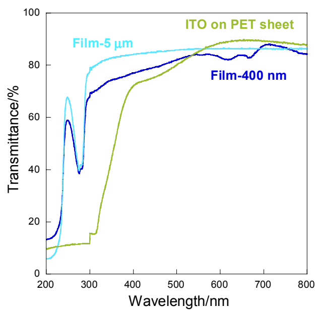
Fig. S1 Transmission spectra of Au nanofin films and ITO on PET sheet.
