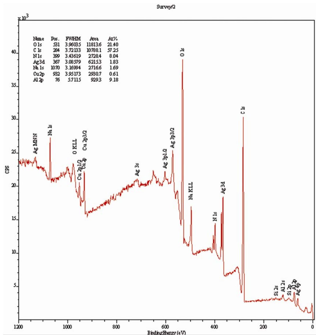
XPS analysis of a dried Cu core Ag shell NPs powder
