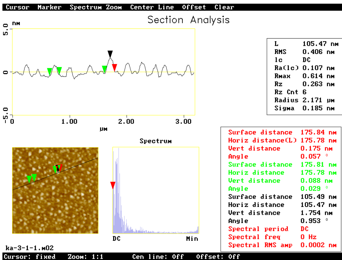
Figure 1 AFM section analysis for mesoporous TiO 2 -loaded SiO x :ZrO x film.
