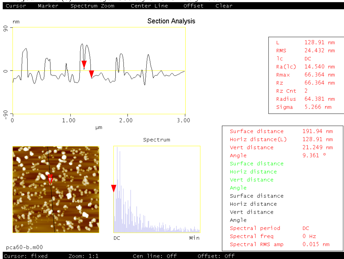
Figure 2 AFM section analysis for of \text{SiO}_x\text{:ZrO}_x film loaded with meso- \text{TiO}_2/(\text{PEI/PSS})_2 containers.
