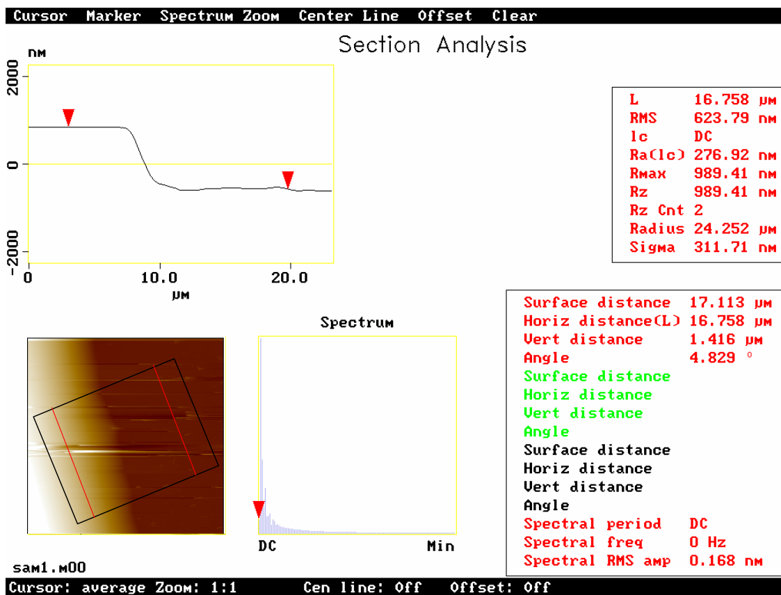
Figure 3 AFM section analysis for edge of TiO 2 -SiO x :ZrO x film.
