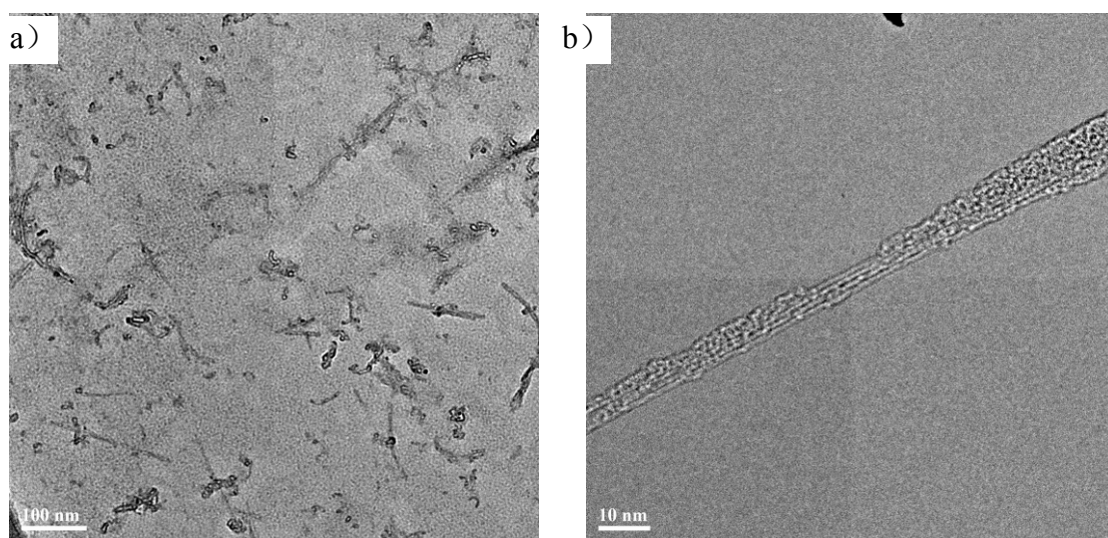
Fig. S2 TEM images of a) shortened SWCNTs and b) short C/S-C.
