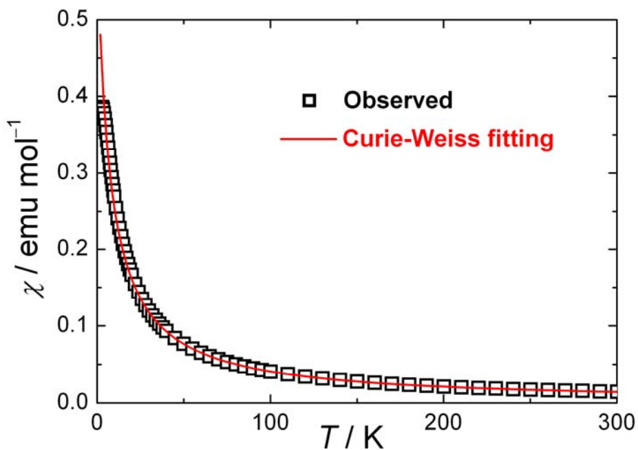
Fig. S1 Temperature-dependent paramagnetic susceptibility ( \chi , black square) of polycrystals of 1 \cdot \text{FeCl}_4 . The red solid line indicates the Curie-Weiss fitting.
