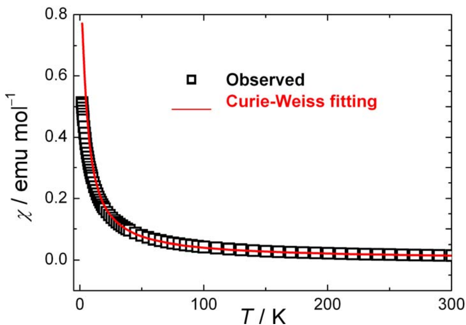
Fig. S2 Temperature-dependent paramagnetic susceptibility ( \chi , black square) of polycrystals of 2 \cdot \text{FeCl}_4 . The red solid line indicates the Curie-Weiss fitting.
