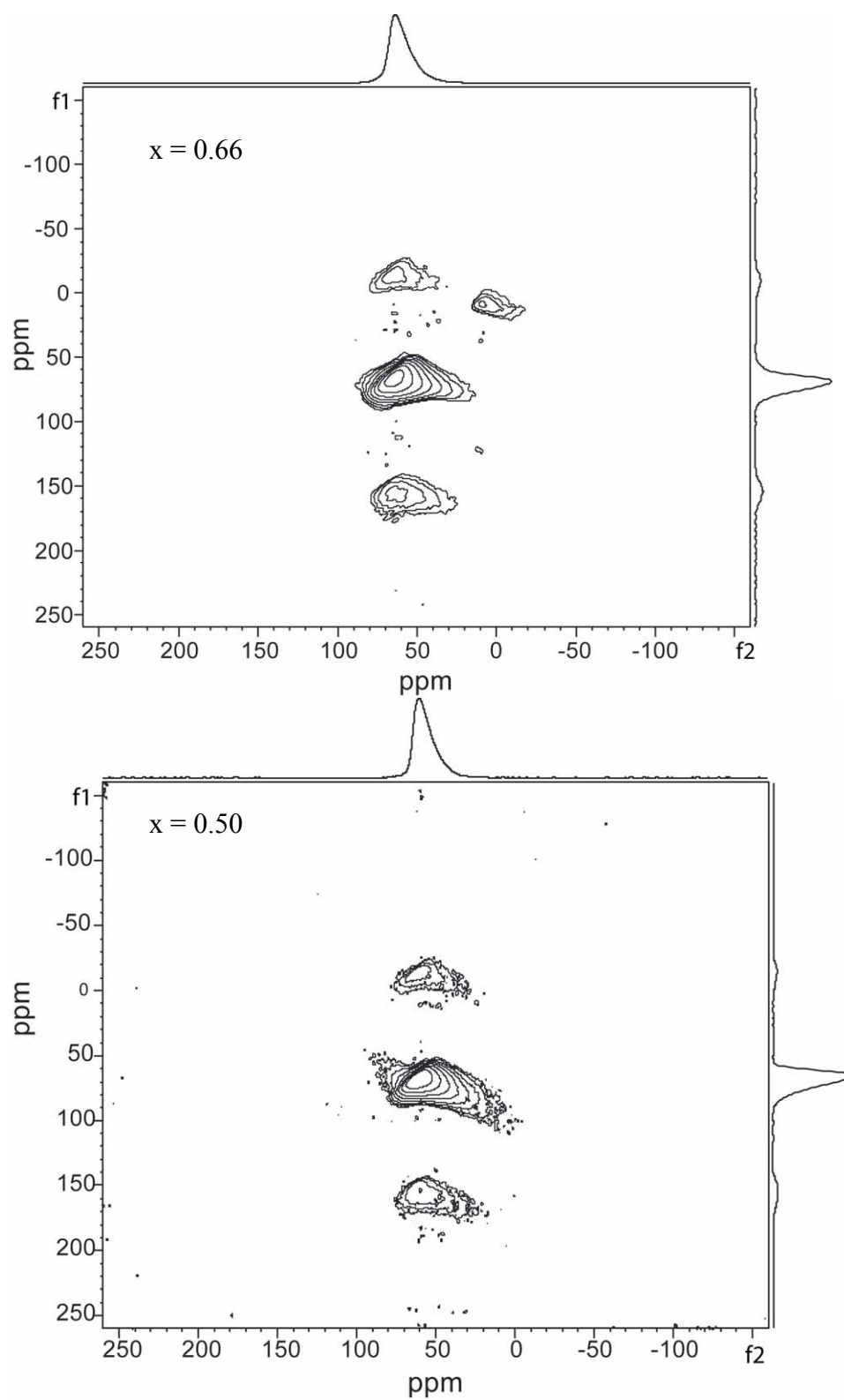
Figure S-I: ^{27}\text{Al} TQMAS spectra of (\text{NaAlO}_2)_x\text{-(SiO}_2)_{1-x}
