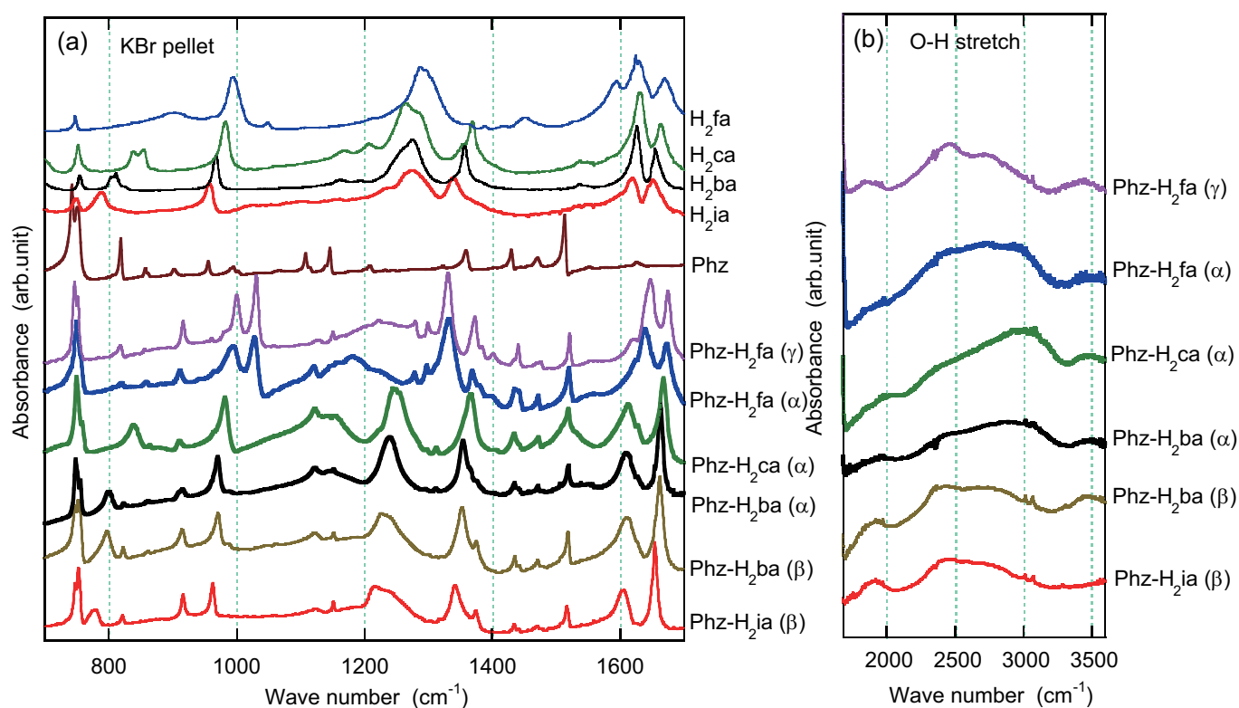
Figure S1 Infrared absorption spectra of powdered Phz-H 2 xa cocrystals in KBr in comparison with those of neutral components.
