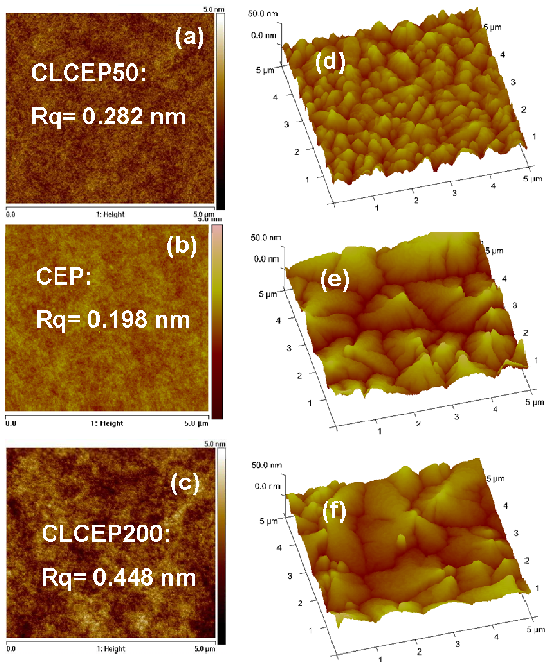
Figure A 5 \times 5 \mu\text{m}^2 AFM images of dielectric surfaces (a) CLCEP50, (b) CEP and (c) CLCEP200, and 60 nm pentacene films grown on (d) CLCEP50, (e) CEP and (f) CLCEP200.
