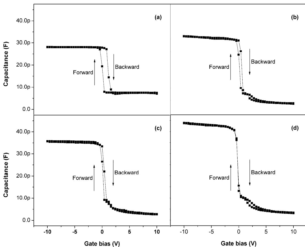
Figure B. Capacitance-voltage (C-V) characteristics of p-Si/CLCEP/Au MIS capacitors with (a) CLCEP50, (b) CLCEP100, (c) CLCEP150 and (d) CLCEP200 as a dielectric.
