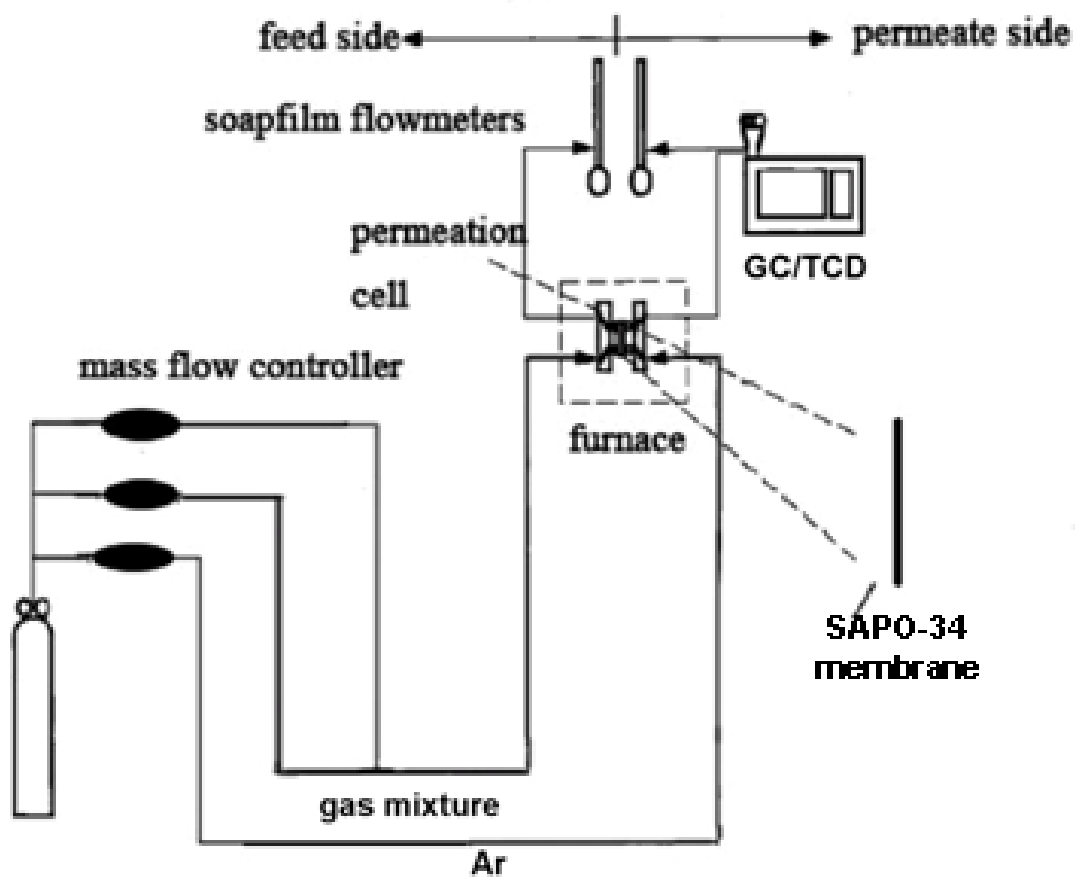
Figure s1. The experimental arrangement for gas-separation measurements with the SAPO-34 membrane at room temperature and at standard atmospheric pressure. One side of the membrane was swept by Ar while the other side was exposed to single gas or gas mixture. A soap-film flow meter is used to measure the flux of the gas and the volume ratio of the mixture gas detected is 1: 1.
