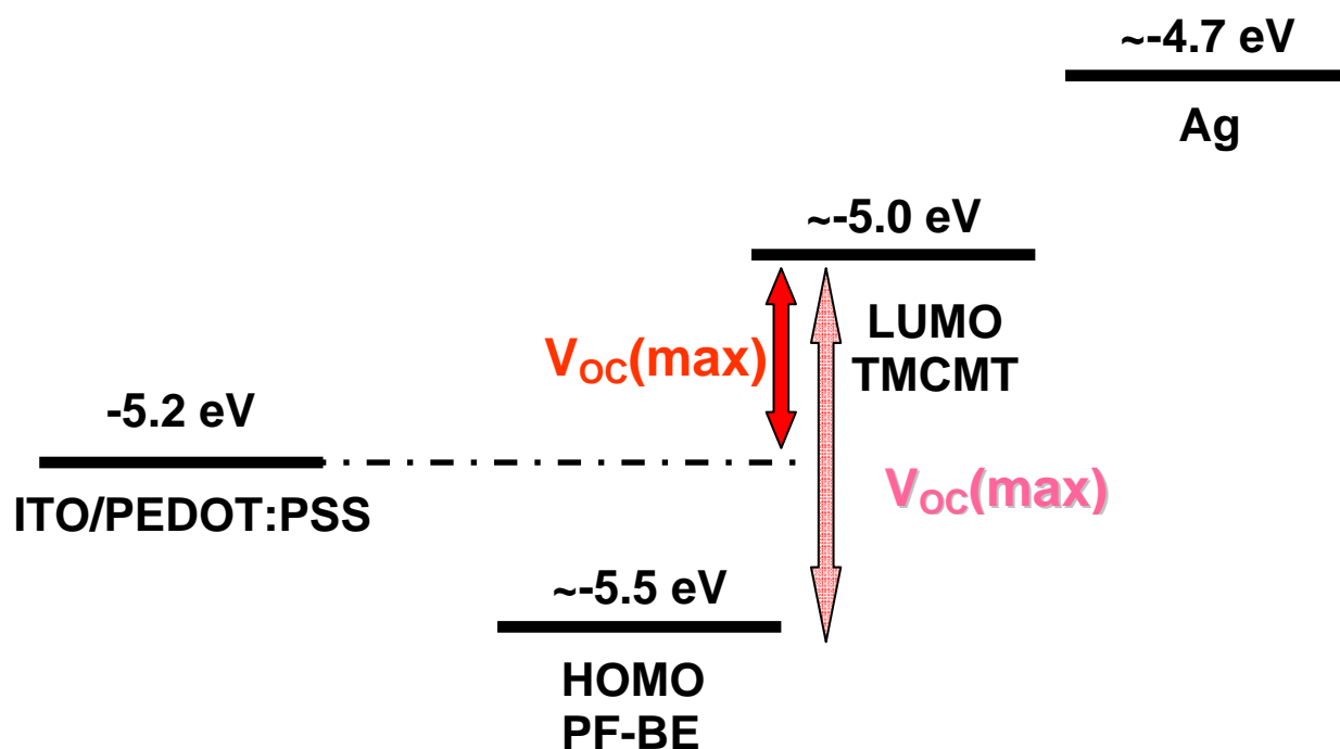
Figure S1. Energy level diagram for the ITO/PEDOT:PSS/PF-BE/TMCMT/Ag system
