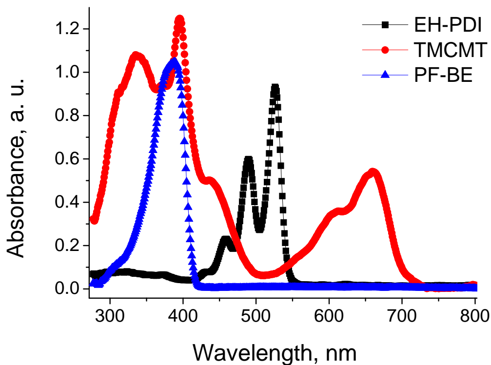
Figure S4. Absorption spectra of the materials measured in dichloromethane
