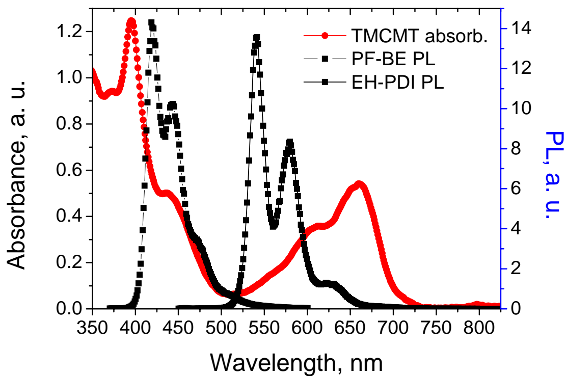
Figure S3. Absorption (TMCMT) and PL (PF-BE, EH-PDI) spectra of the materials measured in dichloromethane
