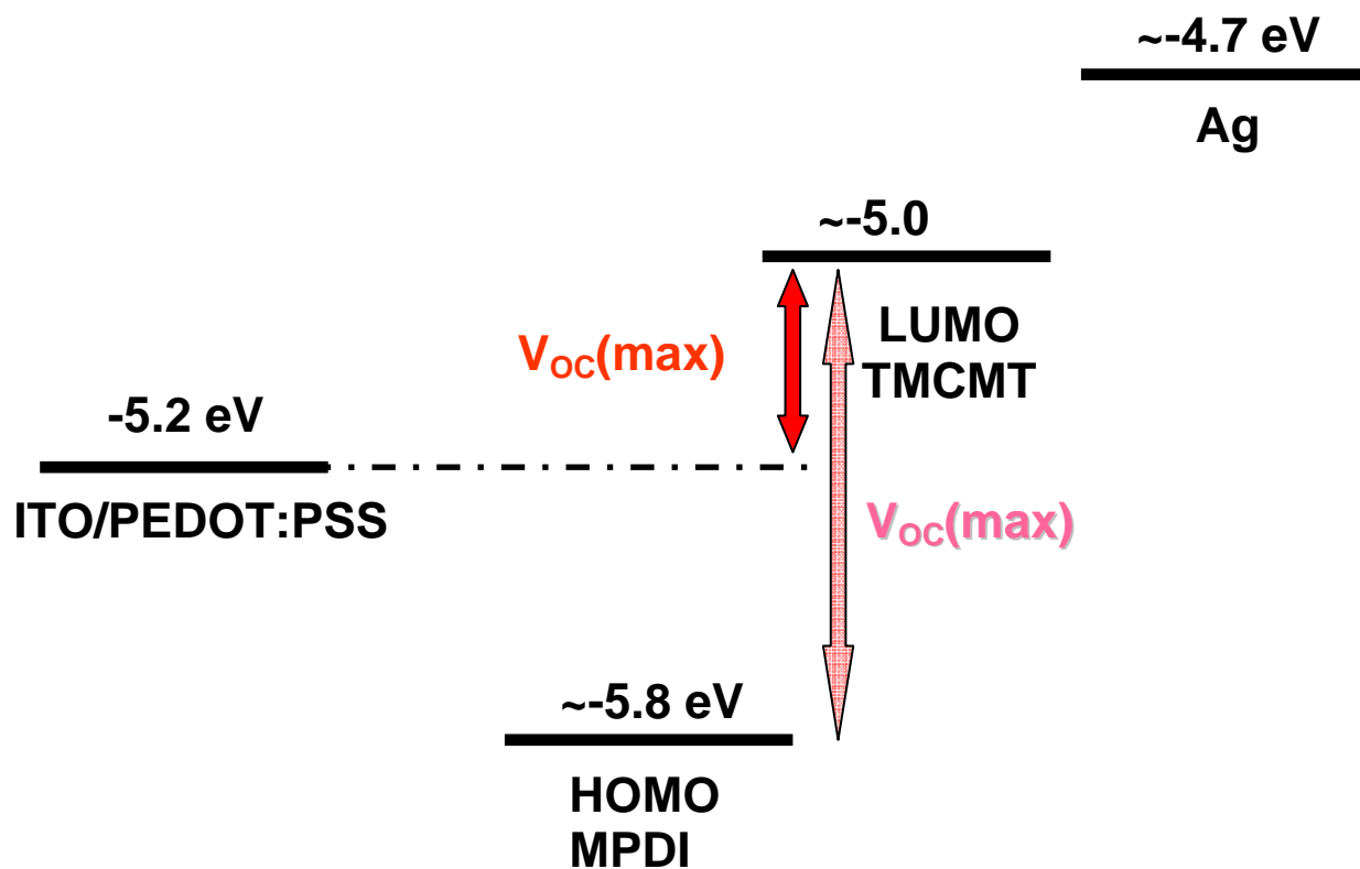
Figure S2. Energy level diagram for the ITO/PEDOT:PSS/MPDI/TMCMT/Ag system
