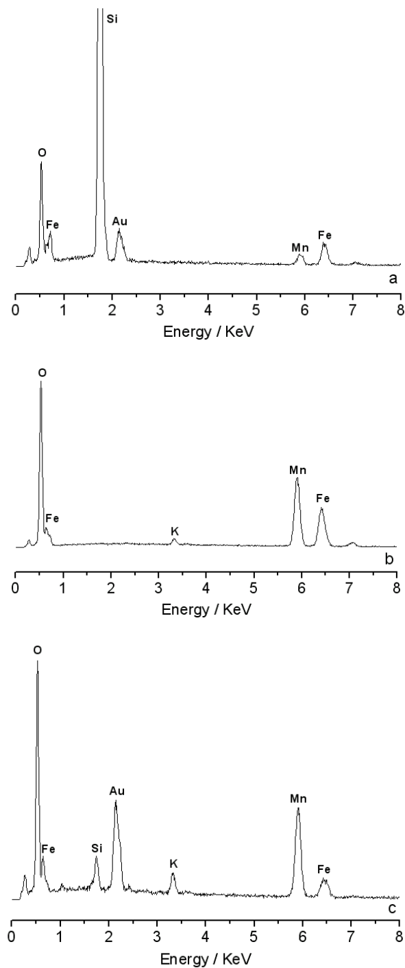
Figure S1. EDX spectra taken on the representative samples (a) sample 1; (b) sample 3; (c) sample 4.
