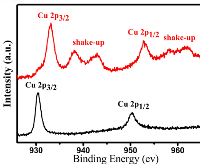
Figure S1. Cu core level X-ray photoelectron spectrum of as-prepared CuSt 2 (red) and Cu 2 S (black).
