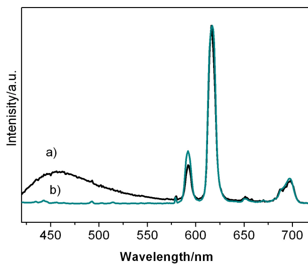
Emission spectra of ionogel Eu@IL-Bipy-SiO 2 (a) and Eu@IL (b), both spectra were obtained 395nm at room temperature.
