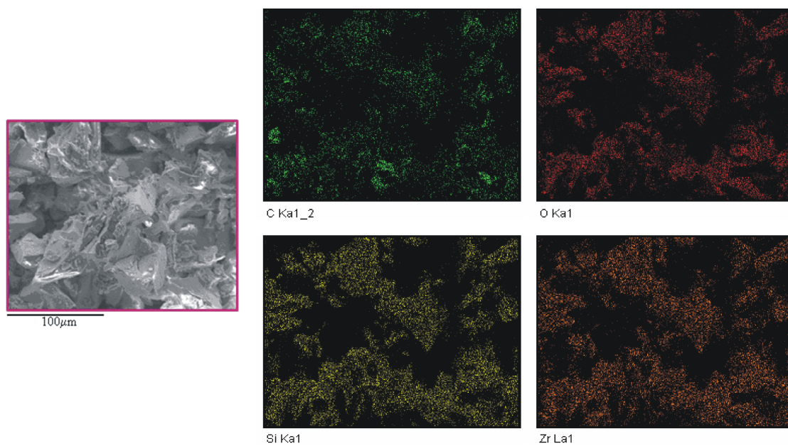
Figure S-2. EDX maps of sample 3F.
