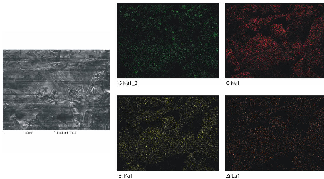
Figure S-1. EDX maps of sample 2F .
