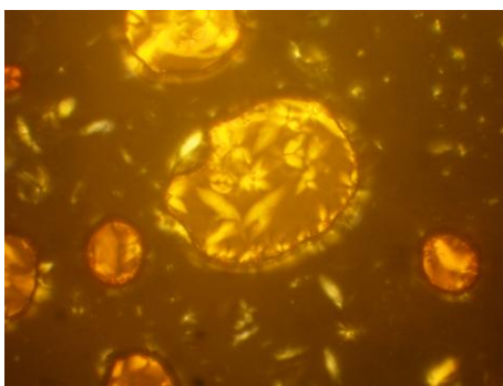
SmA Batonnets growth @ 298°C
