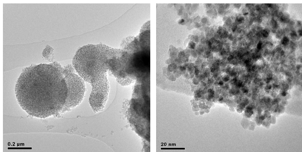
SI Fig.1: TEM pictures of microwave TiO 2 synthesised using butanol at 300W/5min.
