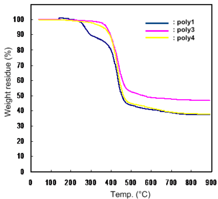
Fig. S4. TGA profiles of poly1 , poly3 , and poly4 .
