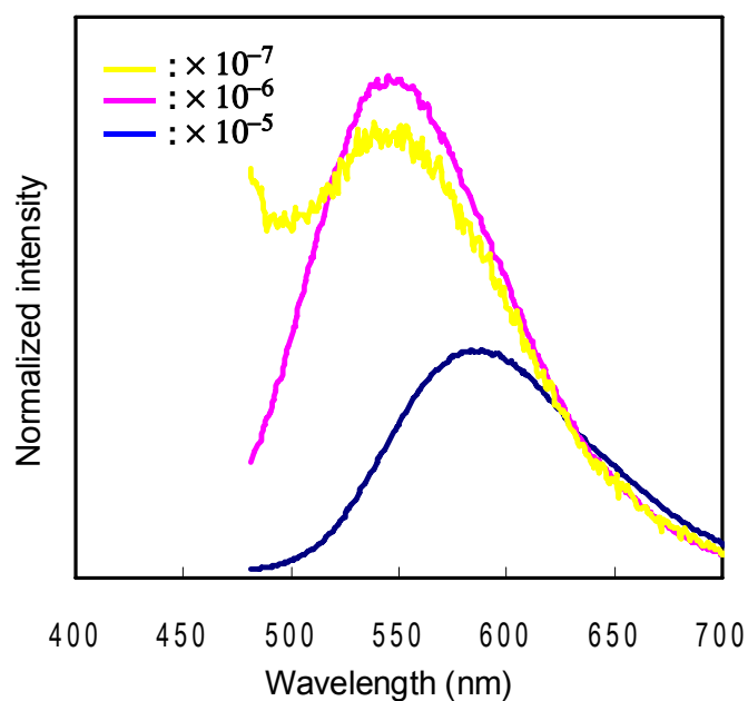
Fig. S3. Normalized PL spectra of poly2 in CH 2 Cl 2 at various concentration ( 10^{-5} ~ 10^{-7} mol/L).
