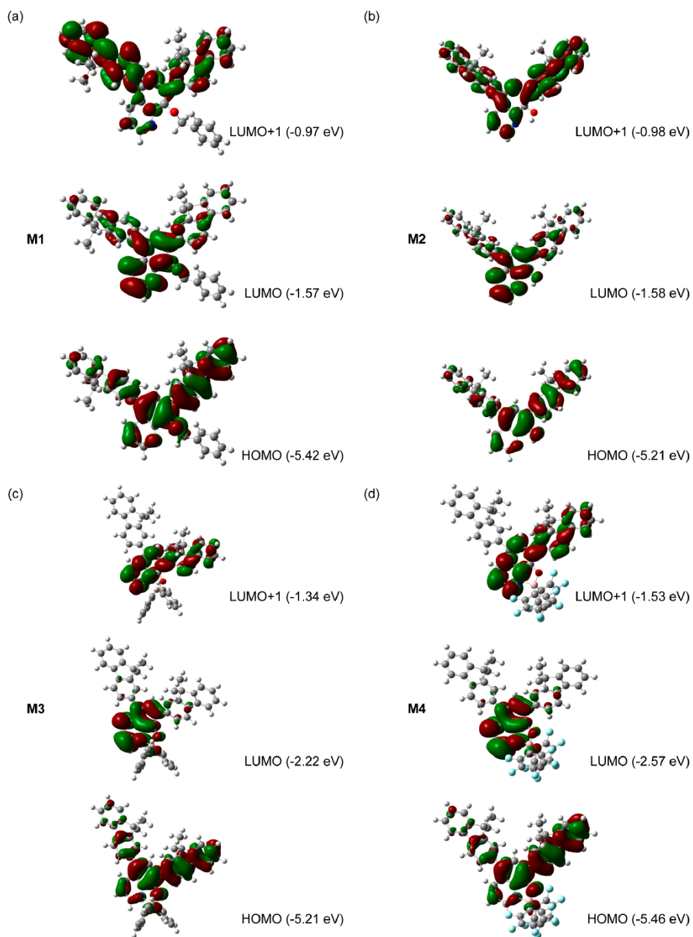
Fig. S5. Molecular orbital diagrams for the LUMO+1, LUMO and HOMO of M1-4 .
