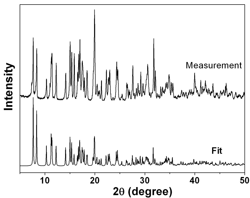
Figure S4 XRD powder pattern of 2 .
