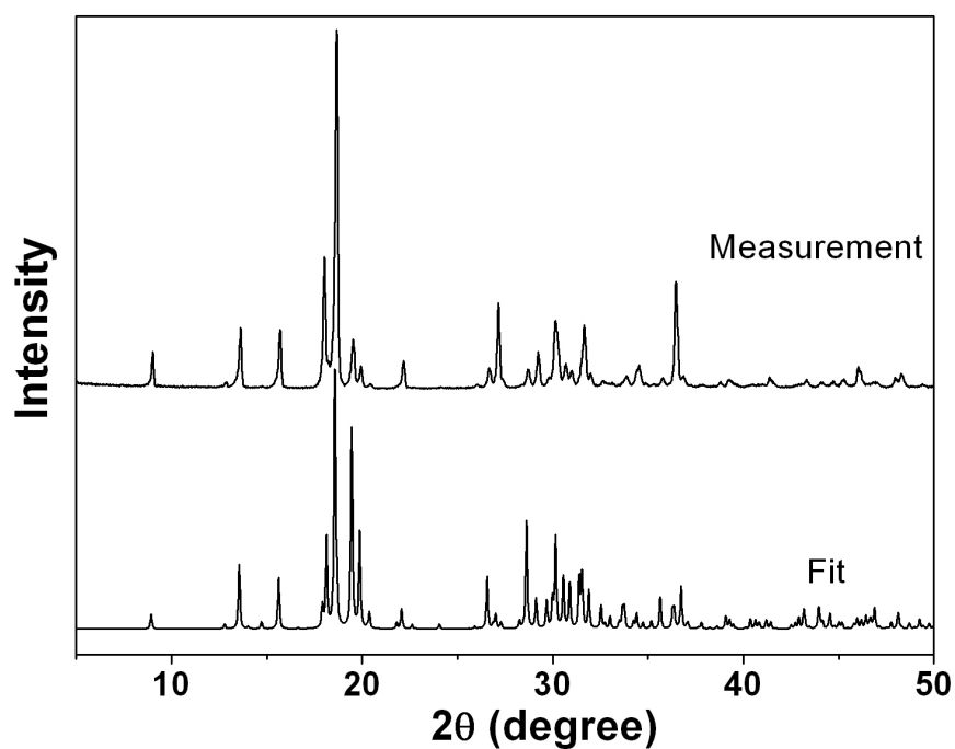
Figure S3 XRD powder pattern of 1 .
