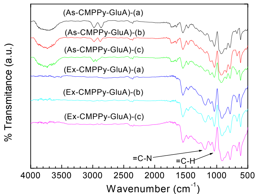
Fig. S1. FTIR spectra of as-synthesized (As-CMPPy-GluA) and copolymer extracted (Ex-CMPPy-GluA) synthesized with PEG 113 -b-poly(GluA) 10 with different concentrations of (a) = 0.75 mmol, (b) = 1.0 mmol, and (c) = 1.25 mmol.
