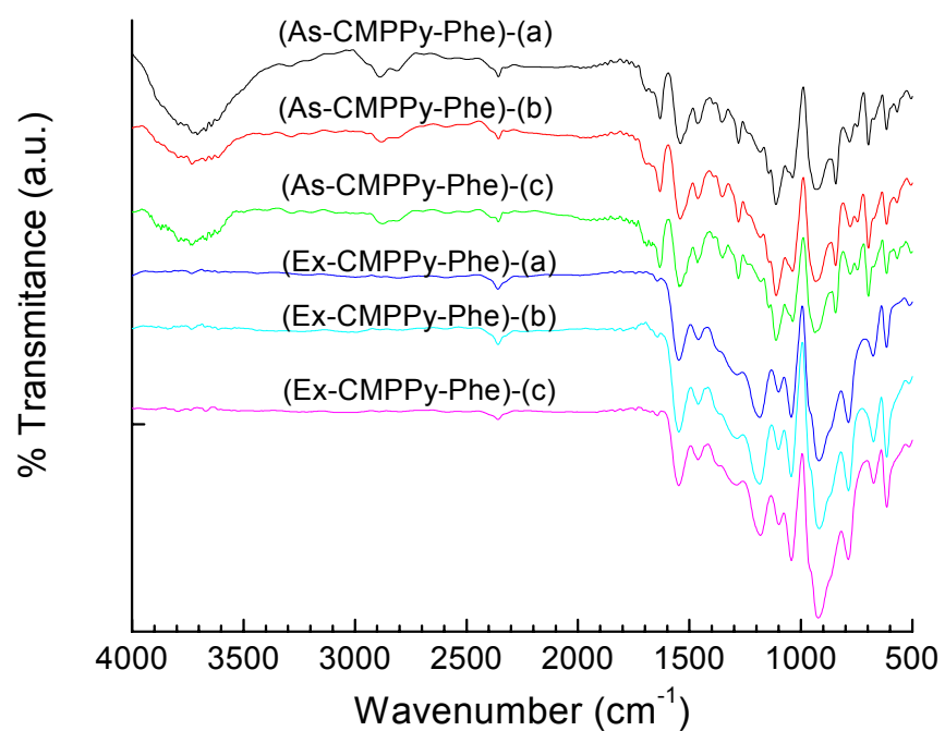
Fig. S2. FTIR spectra of as-synthesized (As-CMPPy-Phe) and copolymer extracted (Ex-CMPPy-Phe) synthesized with PEG 113 -b-poly(Phe) 10 with different concentrations, (a) = 0.75 mmol, (b) = 1.0 mmol, and (c) = 1.25 mmol.
