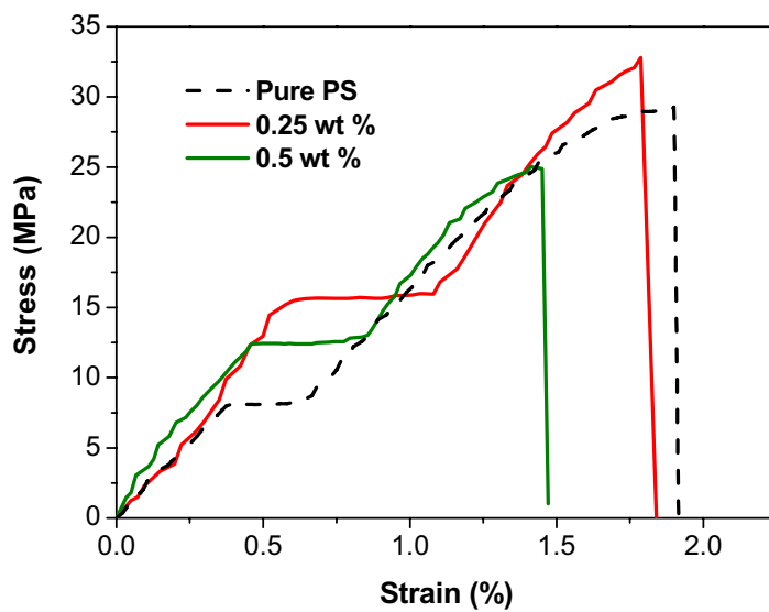
Figure S3. Representative stress-strain curves of pure PS and composites of PS filled with unmodified SiO 2 - h -QDs.
