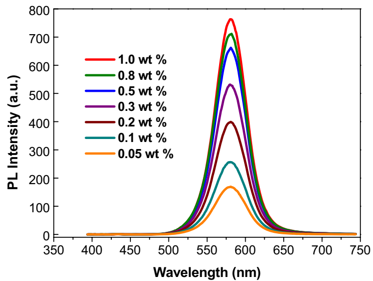
Figure S1. Emission spectra of SiO 2 - h -QD-MSMA/PMMA nanocomposites films filled with different content of SiO 2 - h -QD-MSMAs.
