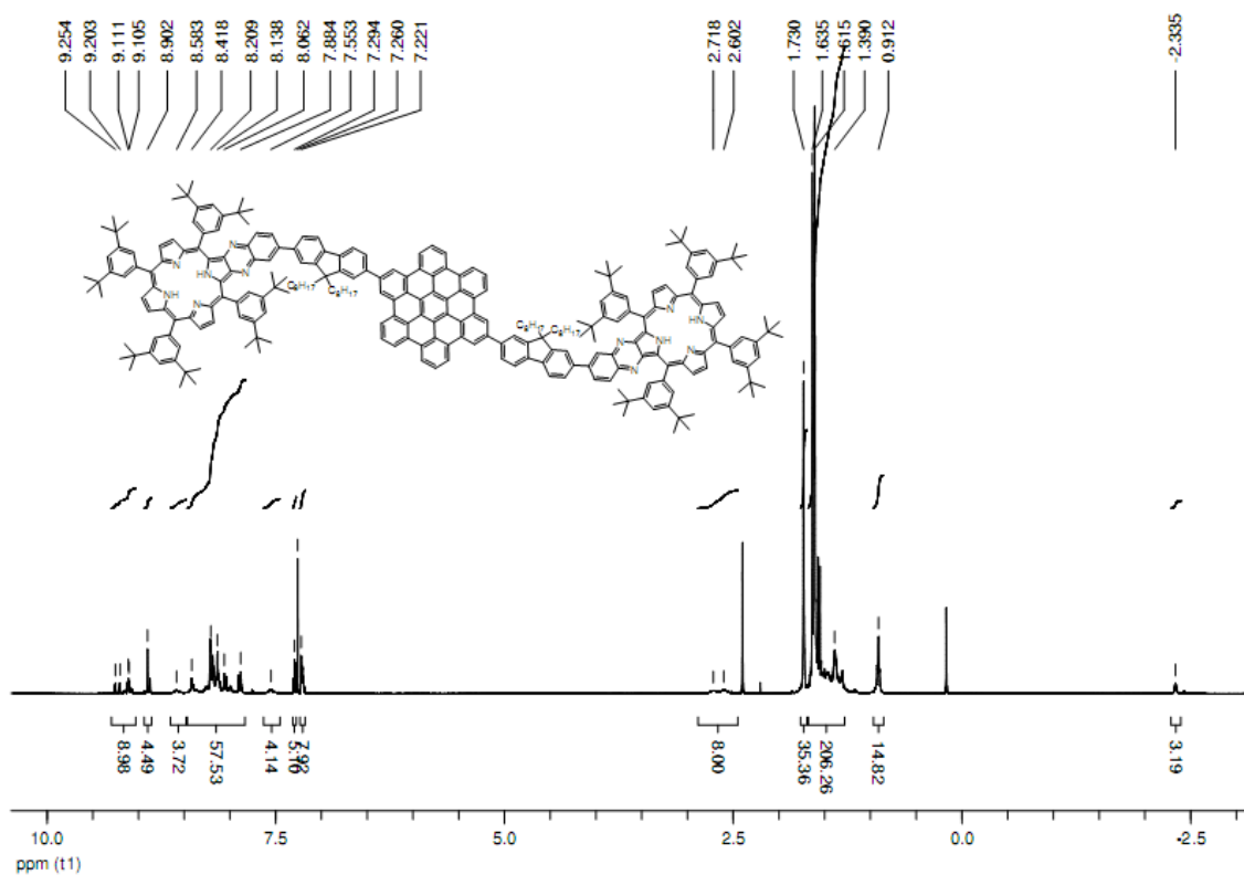
Figure S3. ^1\text{H} NMR (500 MHz) spectrum of compound 6 in \text{CDCl}_3 (20 mM).
