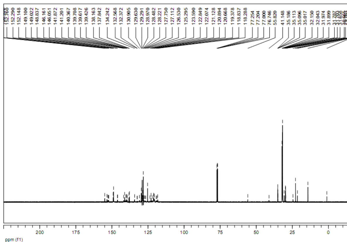
Figure S4. ^{13}\text{C} NMR (125 MHz) spectrum of compound 6 in \text{CDCl}_3 (20 mM).
