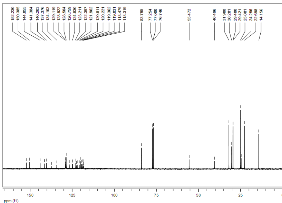
Figure S2. ^{13}\text{C} NMR (125 MHz) spectrum of compound 4 in \text{CDCl}_3 .
