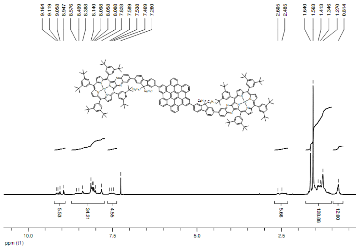
Figure S5. ^1\text{H} NMR (500 MHz) spectrum of compound 6-Zn in \text{CDCl}_3 .
