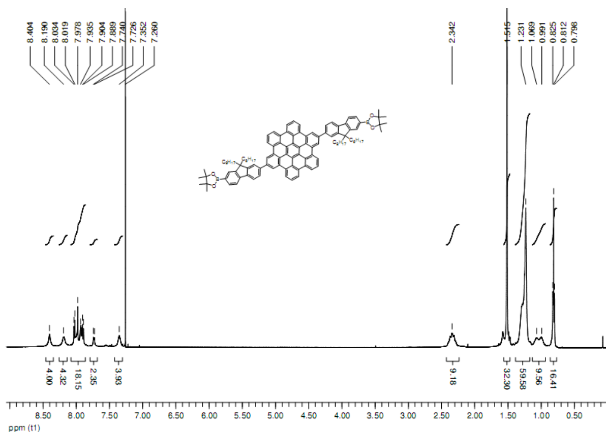
Figure S1. 1 H NMR (500 MHz) spectrum of compound 4 in CDCl 3 .
