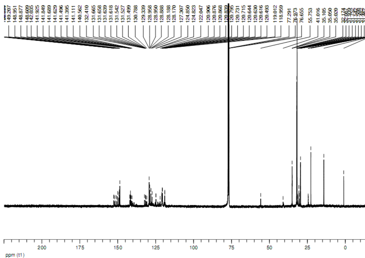
Figure S6. ^{13}\text{C} NMR (125 MHz) spectrum of compound 6-Zn in \text{CDCl}_3 (75 mM).
