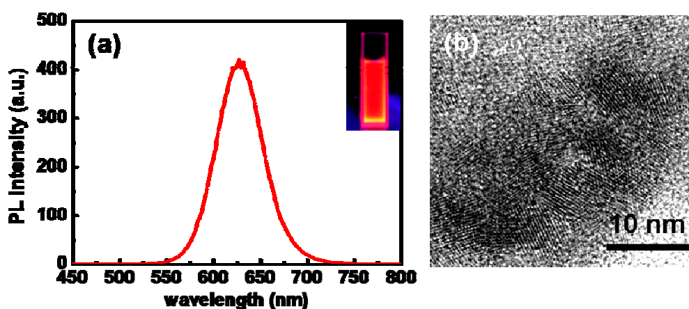
Fig. S1. (a) Photoluminescence emission spectra and fluorescence images of CdTe NCs. (b) High-resolution TEM image of CdTe NCs.
