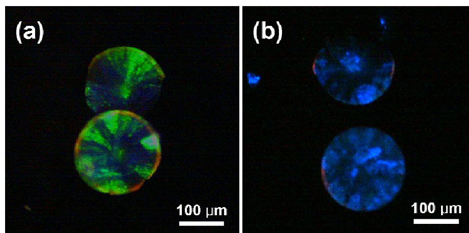
Fig. S2. Cross-sectional optical microscopy images of fluorescent PC supraballs. The cross-section of supraballs exhibit brilliant color of green and blue when they are assembly formed by hybrid microspheres of two different diameters, 230, and 190 nm, respectively.
