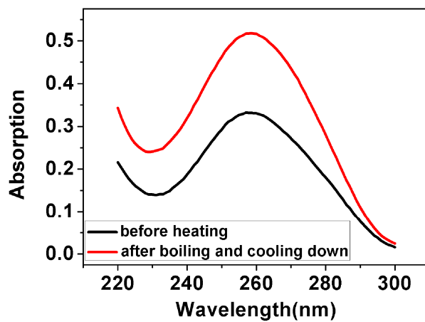
S2 Absorbance spectra of 0.2 mg/mL DNA solutions before heating and after being boiling and cooling down
