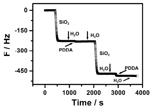
Fig. S2 In situ QCM measurements of alternate deposition of SiO 2 nanoparticles and PDDA.
