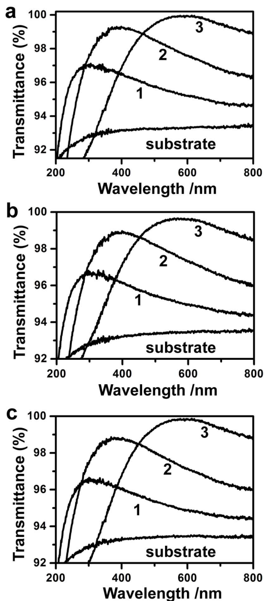
Fig. S1 UV-vis transmission spectra of LbL assembled MSiO 2 /PDDA coatings on quartz substrates fabricated with different dipping times: (a) 5 min, (b) 10 min, (c) 20 min.
