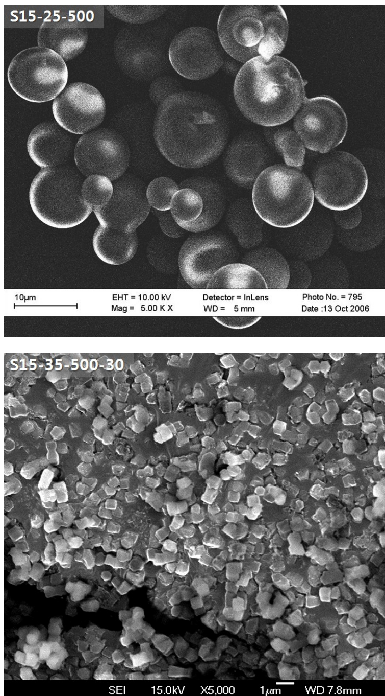
Fig. 1S Low magnification scanning electron micrographs of S15-x-y-(z) samples.
