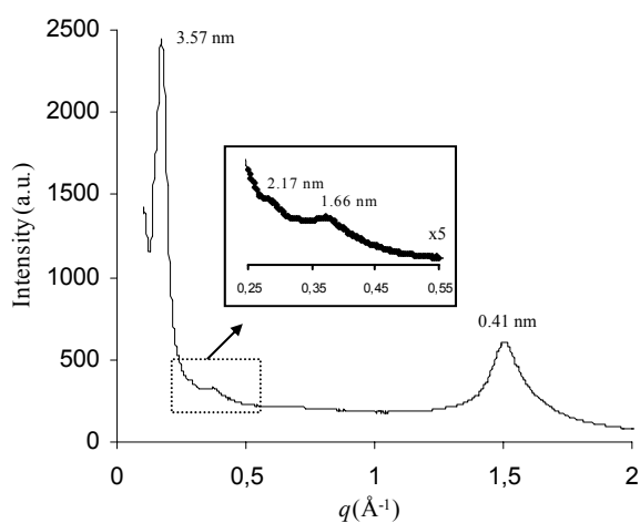
ESI1. XRD pattern of material with 30 carbons. Additional peaks (inset)
