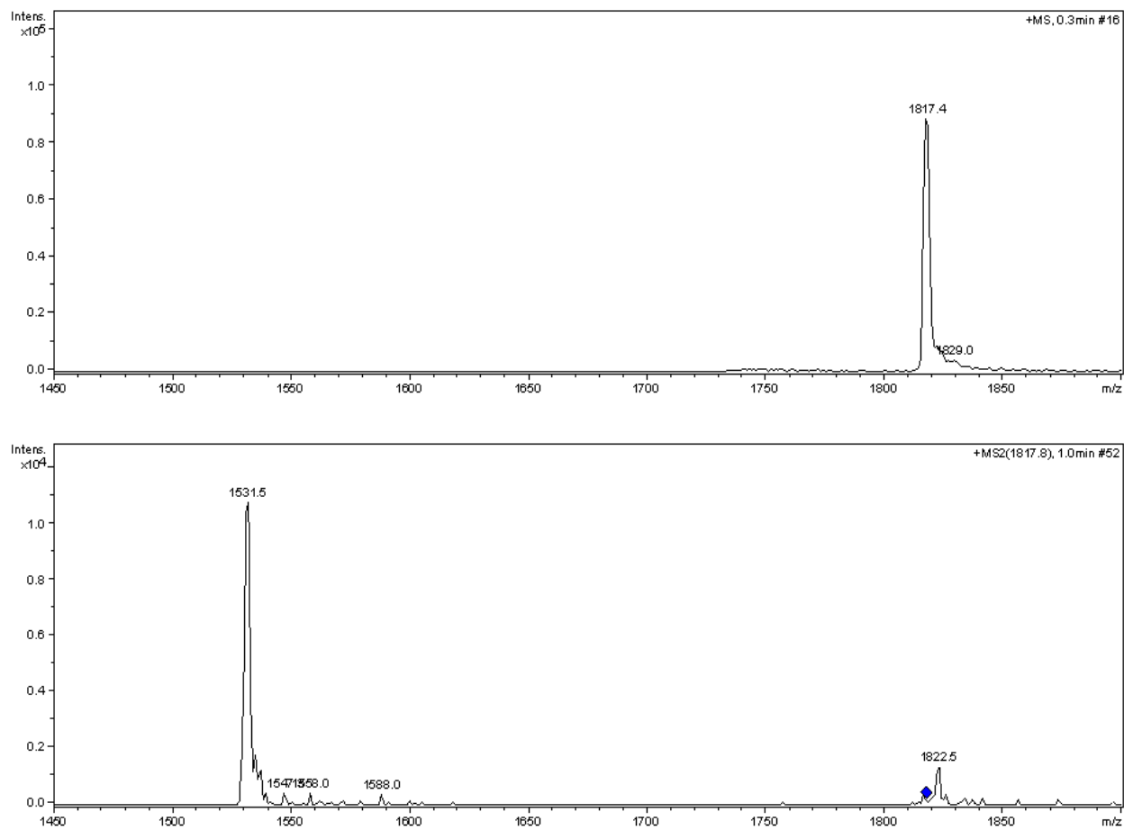
Figure S11: ESI-MS spectrum obtained by the injection of a 5.0 \times 10^{-5} mol/L, \text{CH}_2\text{Cl}_2 solution of TTIP and its MS 2 fragmentation products obtained by the entrapment of 1817 m/z ion.
