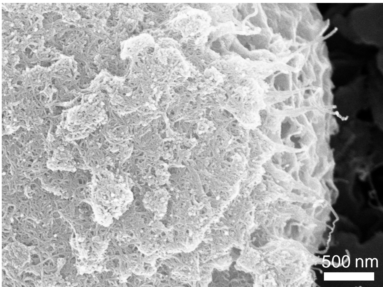
Figure S1. An enlarged SEM image of HAp mineralized with CNT-PDA for 7 days. HAp agglomerates were highly intercalated with a network of CNT-PDA nanofibers.
