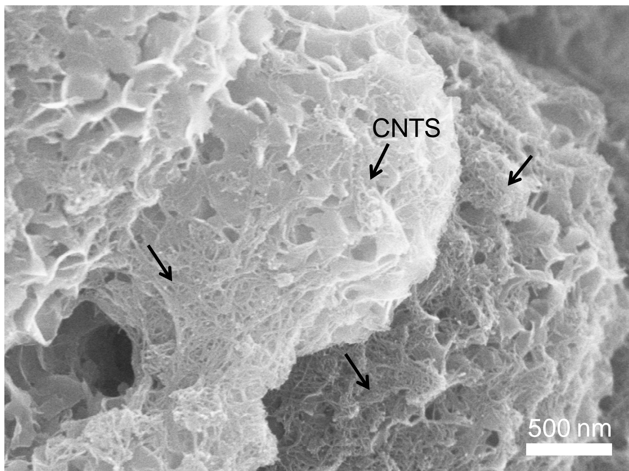
Figure S2. An enlarged SEM image of HAp mineralized with CNT-PDA for 7 days. HAp minerals were successfully developed with an intercalating CNT-PDA network, as indicated with black arrows.
