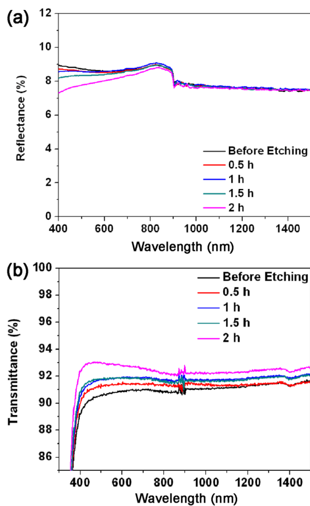
Figure S2. (a) Reflectance spectra of glass C before and after etching. (b) Transmittance spectra of glass C before and after etching.
