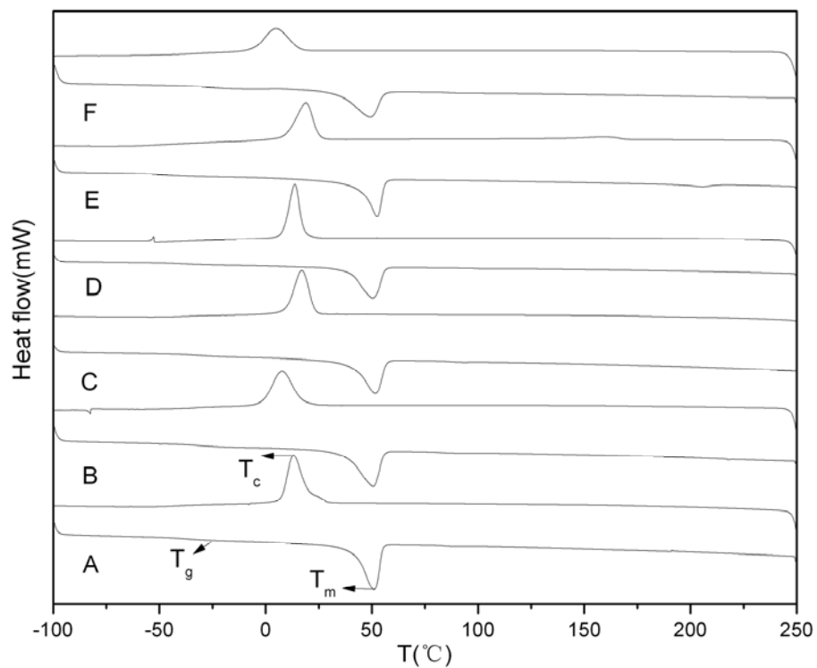
Fig.S3 DSC curves second heating and cooling of azoPU and PU (samples A-F)
