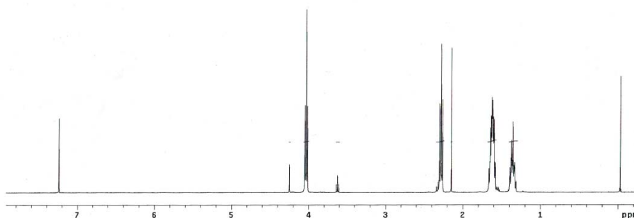
Fig.S1 ^1\text{H} NMR spectrum of PCL in \text{CDCl}_3
