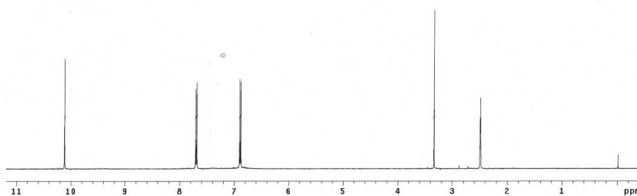
Fig.S2 ^1\text{H} NMR spectrum of 4, 4'-dihydroxyazobenzene in \text{CDCl}_3
