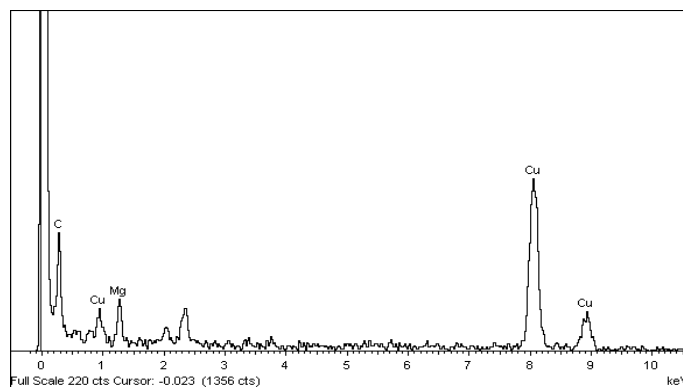
Fig. S2 Energy dispersive X-ray (EDX) spectrum of mesoporous MgO/carbon composites MC-600-0.15.
