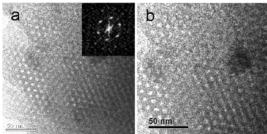
Fig. S1 TEM images of mesoporous MgO/carbon composites MC-600-0.3 (a) and MC-600-0.4 (b).
