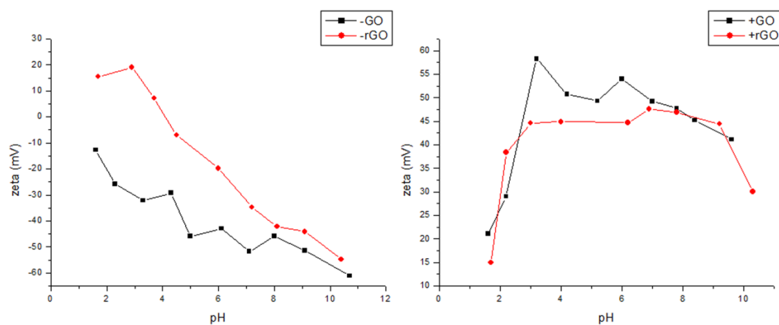
Figure S1. Zeta potentials at different pH values for negatively charged GO and rGO and positively charged GO and rGO solutions. Concentration of each solution is 0.005 wt%.
