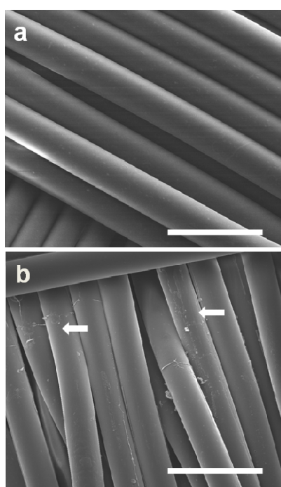
Fig. S1 SEM images of textile fibers coated with a) crosslinked coating C8, and b) un-crosslinked PDMAMS after the durability test. Scale bar is 50 \mu\text{m} . White arrows indicate the debris of the PDMAMS coating.
