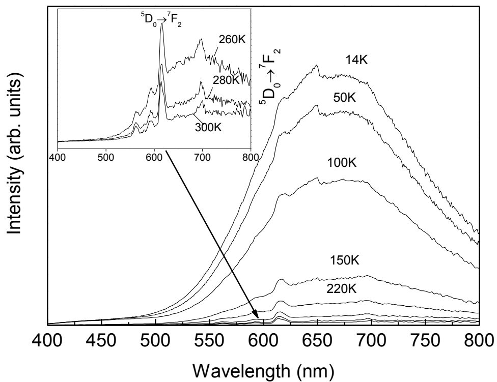
Figure S1. Emission spectra of the Eu 3+ -doped CdS NCs excited at 280 nm in the temperature interval 14-300 K. For a better visualization, the inset shows a magnification of the 260, 280 and 300K spectra.
