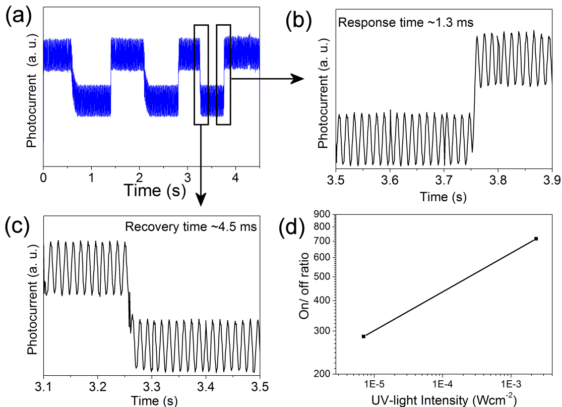
Figure S1 (a)-(c) Response curve and recovery curve, as time-resolution increased to 1 kHz, under UV-light ( 7\mu\text{Wcm}^{-2} ) irradiation. (d) The UV-light intensity dependence of the photoresponse.
