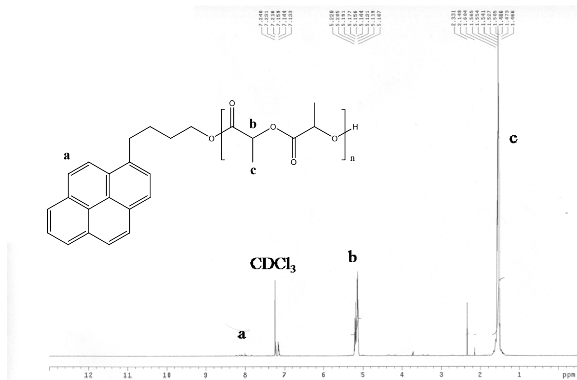
Figure S1. 1 H NMR spectrum of pyrene-labeled PLA
