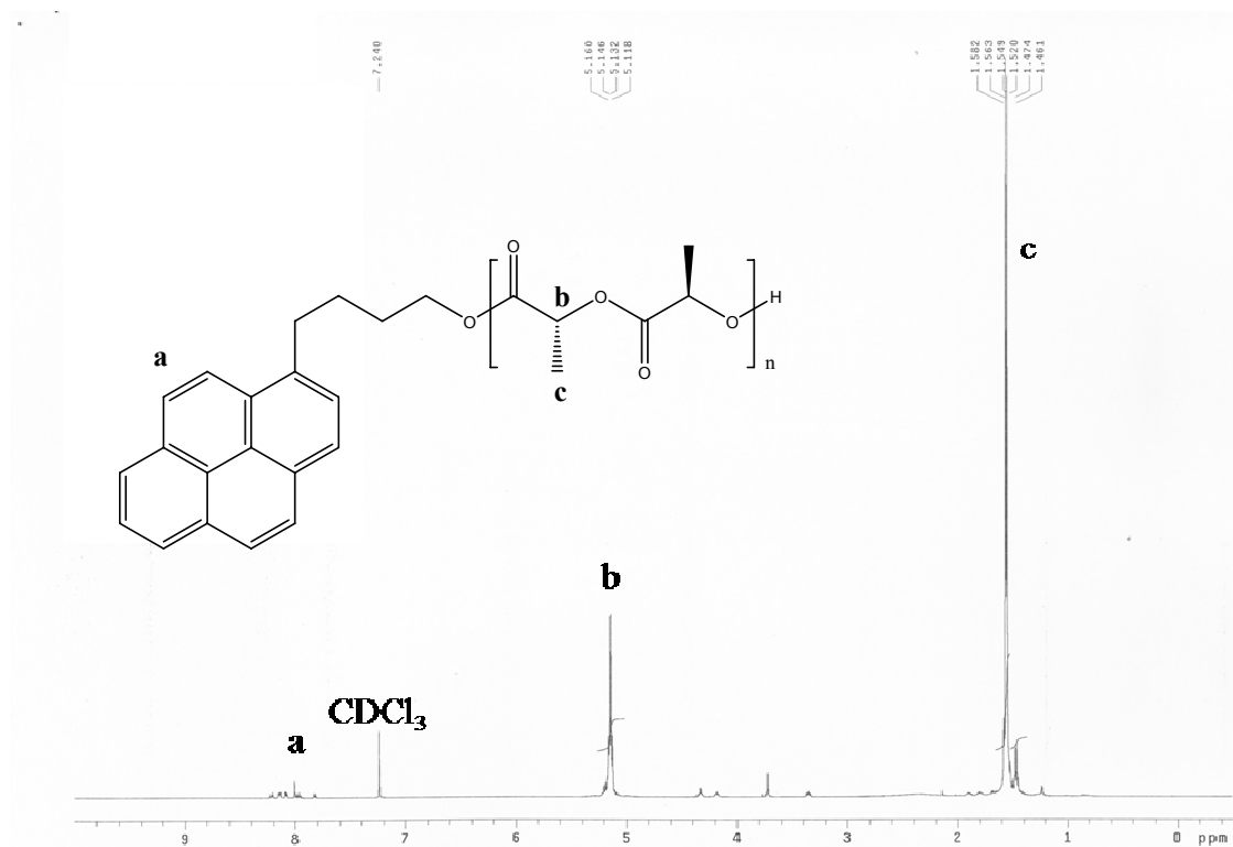
Figure S3. 1 H NMR spectrum of pyrene-labeled PDLA
