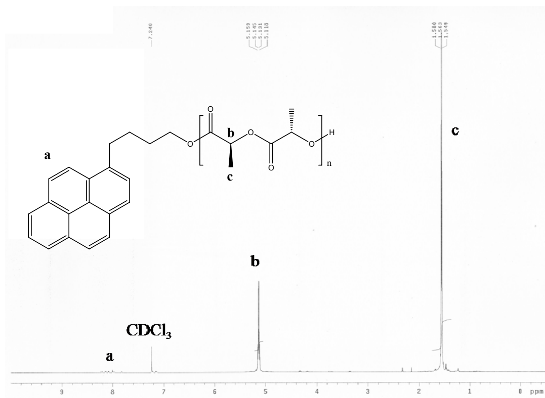
Figure S2. 1 H NMR spectrum of pyrene-labeled PLLA
