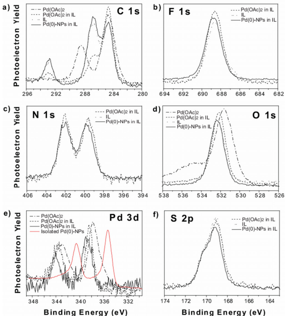
Fig. 3 XPS analyses of palladium in IL.
