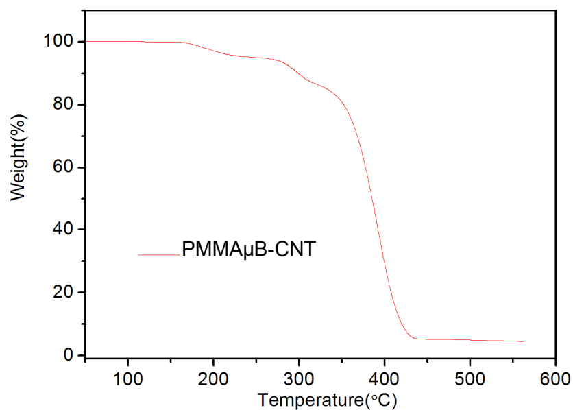
Figure 11: TGA curves of CNT-d-PMMA \mu B
