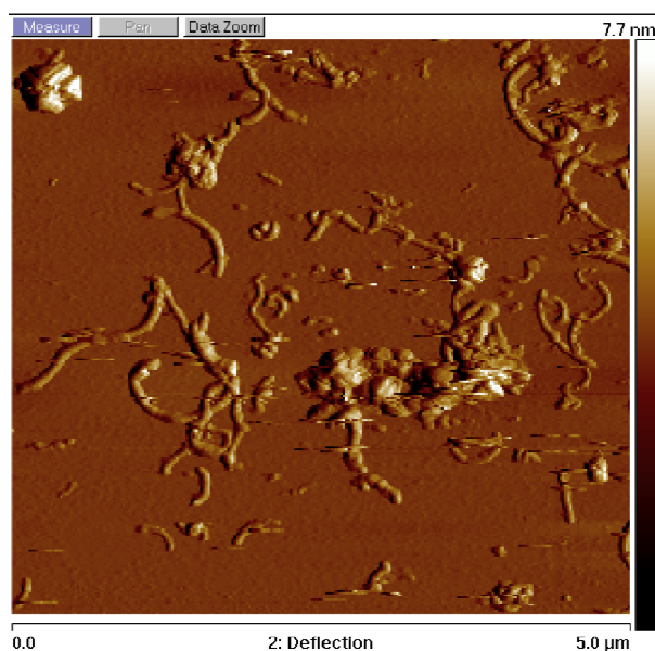
Figure 12: AFM characterization of CNT used in this study
