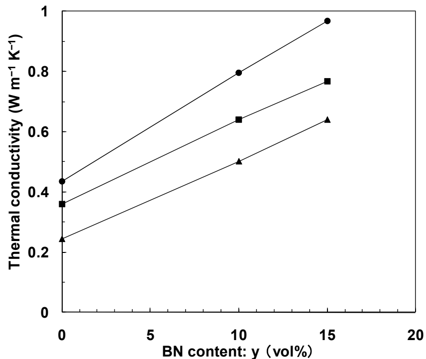
Supplementary Fig. 1 Thermal conductivity of PPS/BN ((100-y) %/y vol%) composites (▲), MWCNT/PPS/BN ((100-y)×0.01 vol%/(100-y)×0.99 vol%/y vol%) composites (■) and MWCNT/PPS/PE/EGMA/BN ((100-y)×0.01 vol%/(100-y)×0.71 vol%/(100-y)×0.21 vol%/(100-y)×0.07 vol%/y vol%) composites (●).
